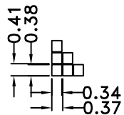
DOT DETAIL SCALE 5:1
